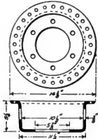
Figs. 4149-4150. Wash-out Well.
